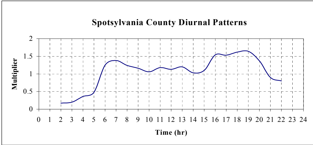
Figure 2 – Water Demand Hourly Diurnal Pattern
