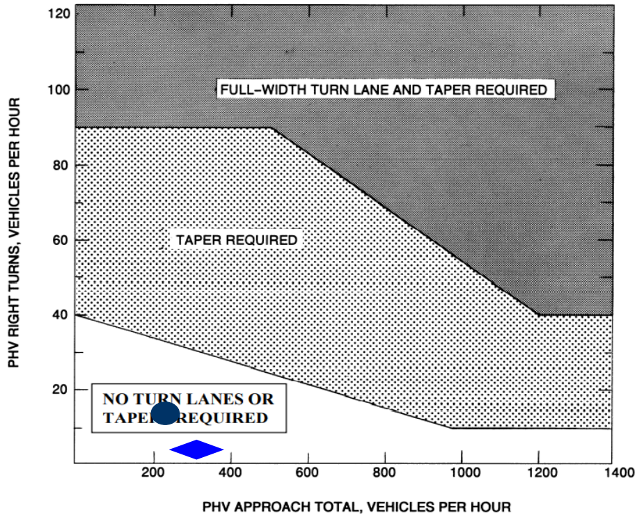
FIGURE 3-27 WARRANTS FOR RIGHT TURN TREATMENT (4-LANE HIGHWAY) Source: VDOT RDM, Appendix, F, Figure 3-27 (Page F-90), Calculations by Pennoni
